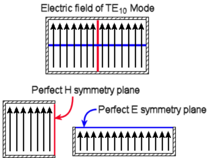
Figure 4-6: Electric Field and Symmetry planes
