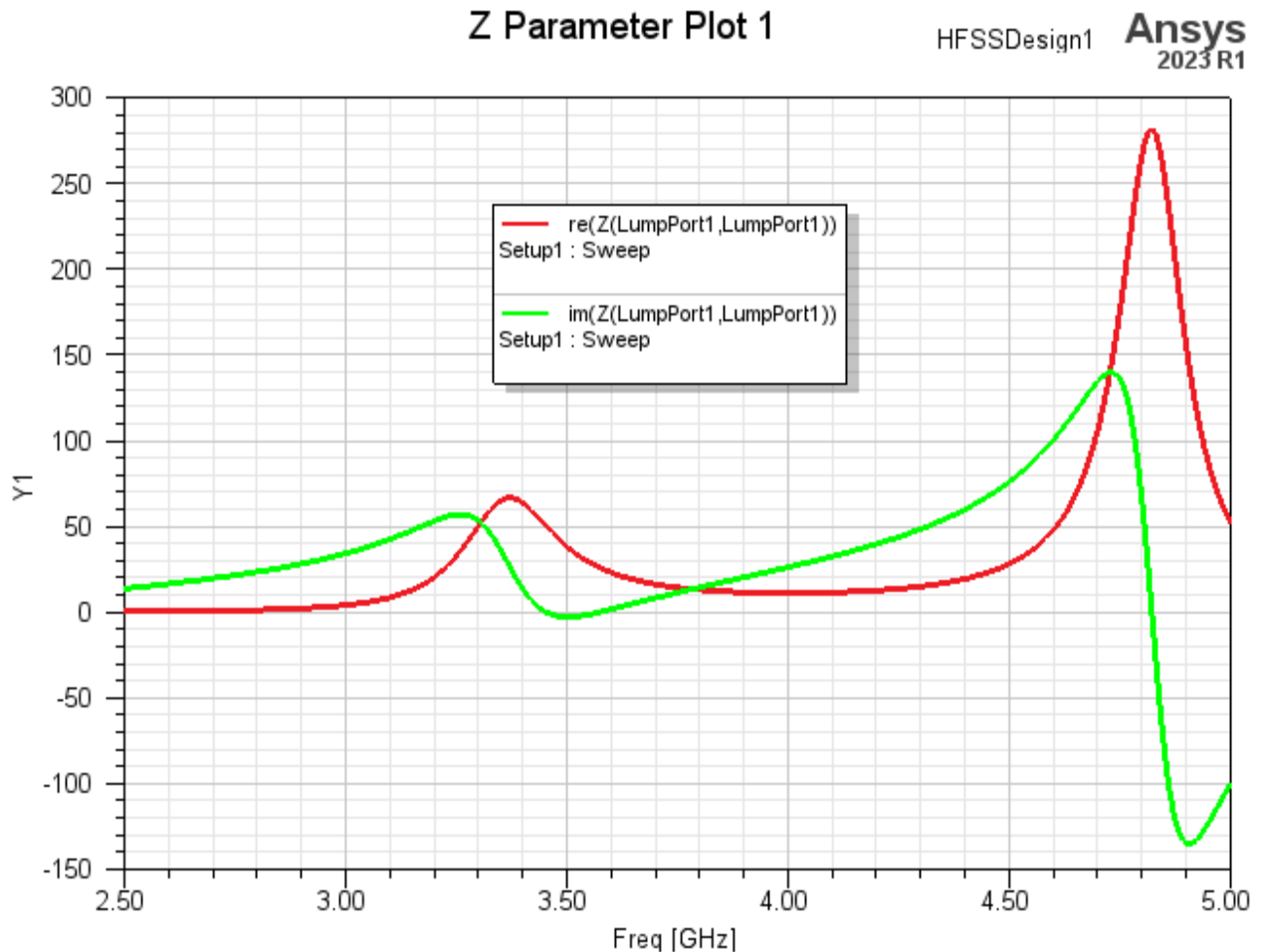
Figure 6-3: Z Parameter Plot 1 – Z(\text{LumpPort1}, \text{LumpPort1}) , Real and Imaginary Traces
