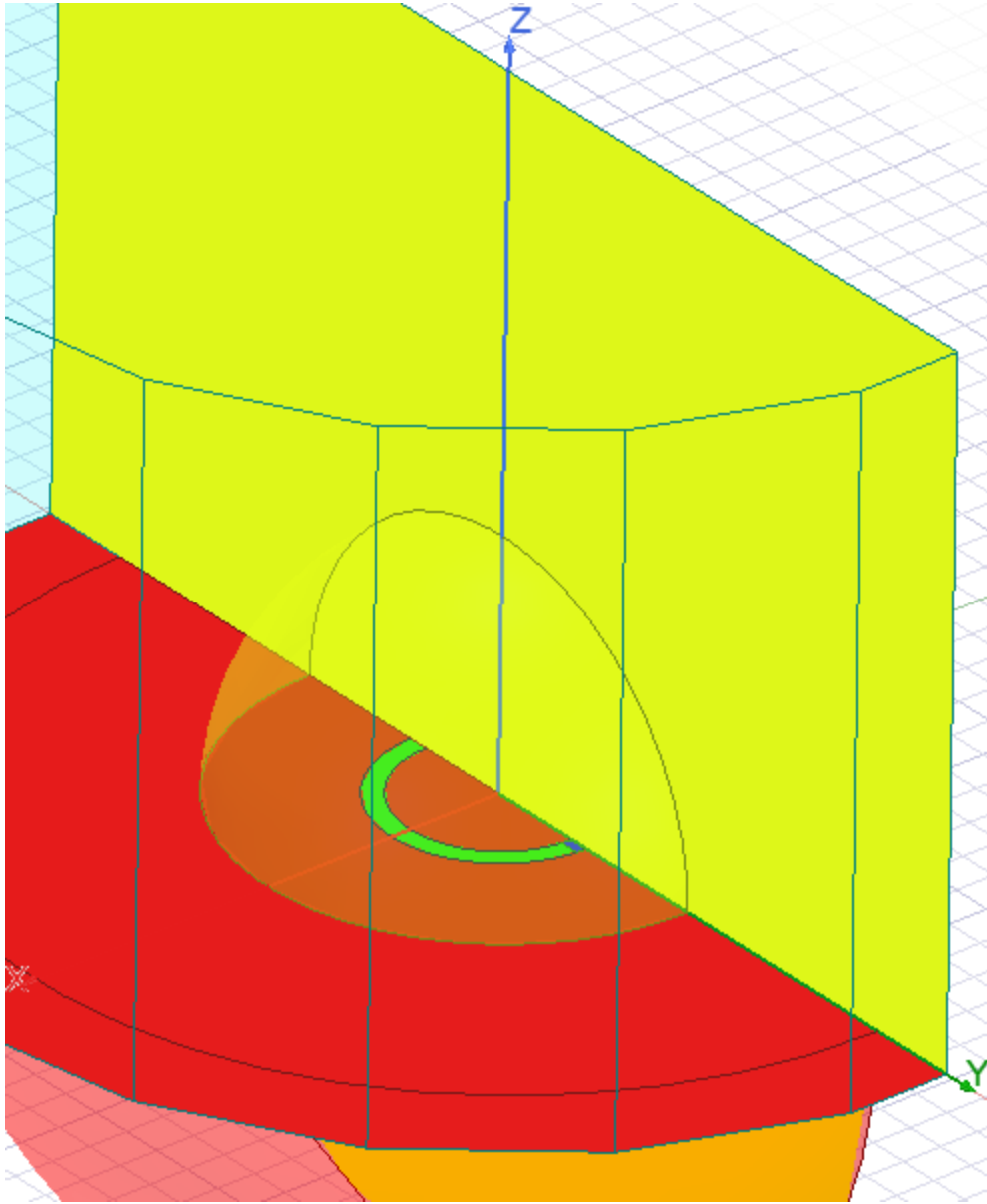
Figure 4-16: Solver View of Boundaries – PerE1 , PerfH1 , Sym1 , and LumpPort1 Selected
