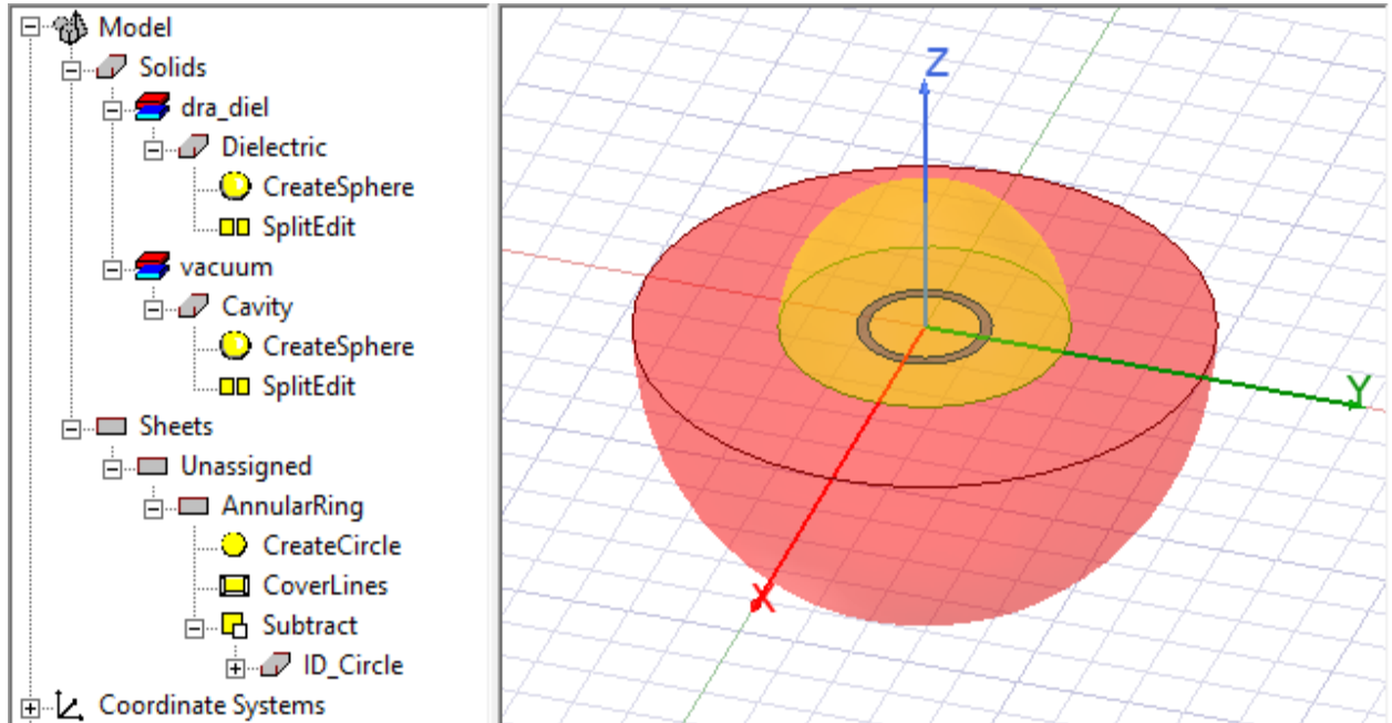
Figure 3-19: AnnularRing Completed
